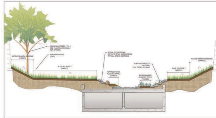
Exhibit 3: Channel Cross Section Showing Stormwater Conveyance Box
