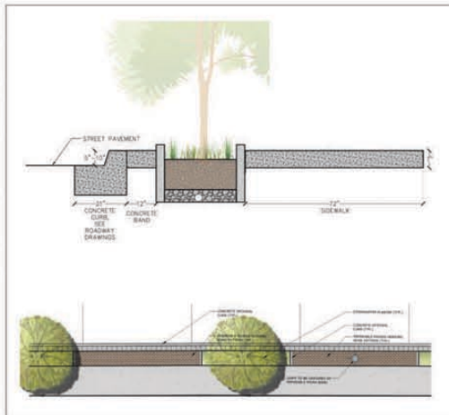
Exhibit 2: Typical Stormwater Planters
